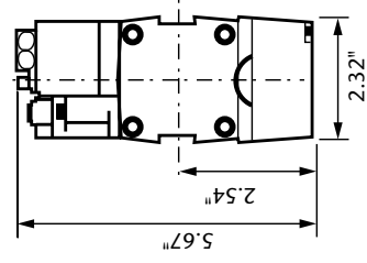
AFD215 pneumatic drive
