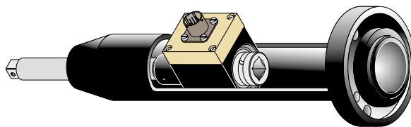
TRANSDUCER-HOLDER FROM EM TOOL PART NO With 3/8" square drive 615 396 119 0 With 1/2" square drive 615 396 120 0
