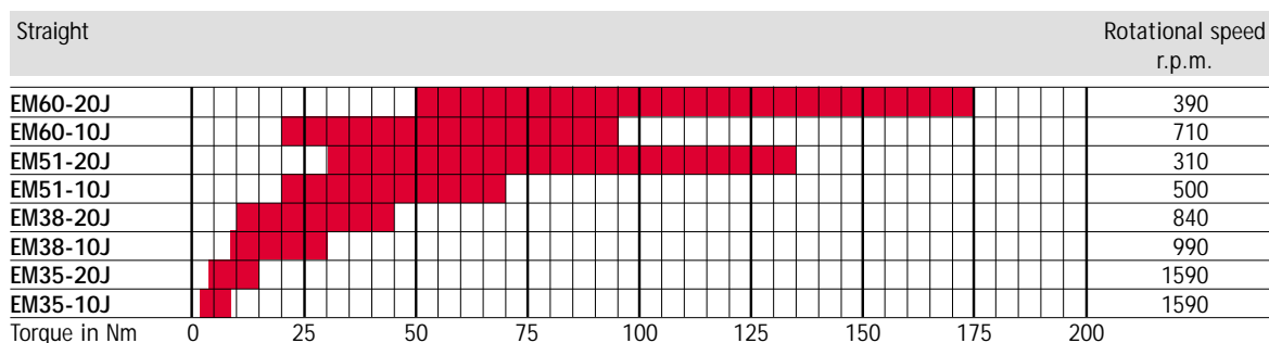
Performances of fixed electric tools series "EM" and "EML"
