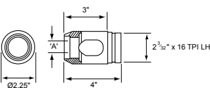
Nose Attachment 3
