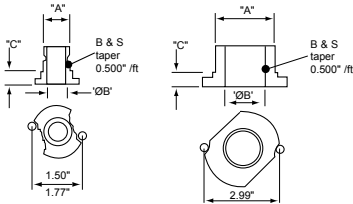
Nose Attachment 1
