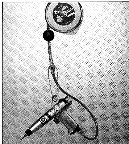
A suspension clip and hose assembly is available for pistol grip tools. Part N° 107403 (3HU, 4HU). Part No 115193 (4HI).
